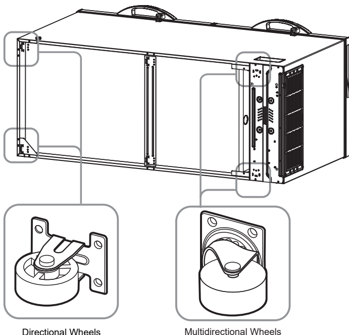
Directional Wheels
