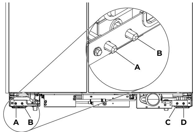
A. Rear leveling bolt B. Front leveling bolt C. Rear leveling bolt D. Front leveling bolt
