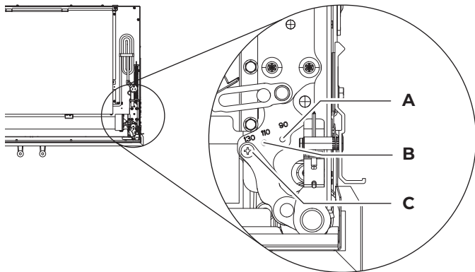
A. 90° position B. 110° position C. 130° position door swing adjustment screw
