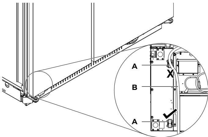
A. Rollers wheels B. Water supply line
