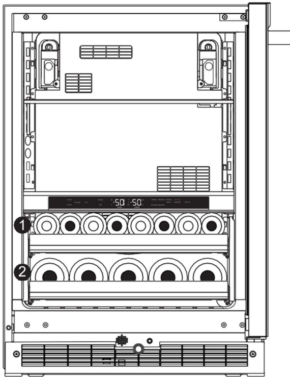
Rack 1: For storing up to eight 750 ml wine bottles [diameter less than or equal to 3 1/8" (80 mm)] Rack 2: For storing up to five larger wine bottles [diameter up to 3 3/4" (95 mm)]
