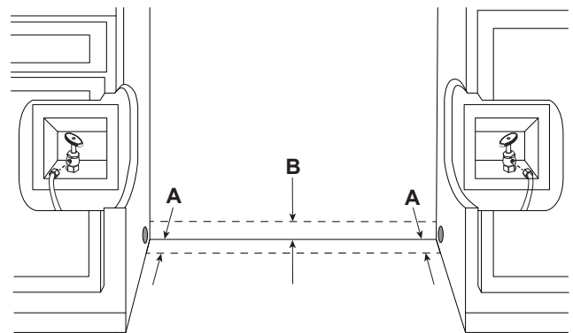
A. Waterline access hole to be within 1/2" (13 mm) from back wall. B. Waterline access hole to be within 1/2" (13 mm) from floor.
