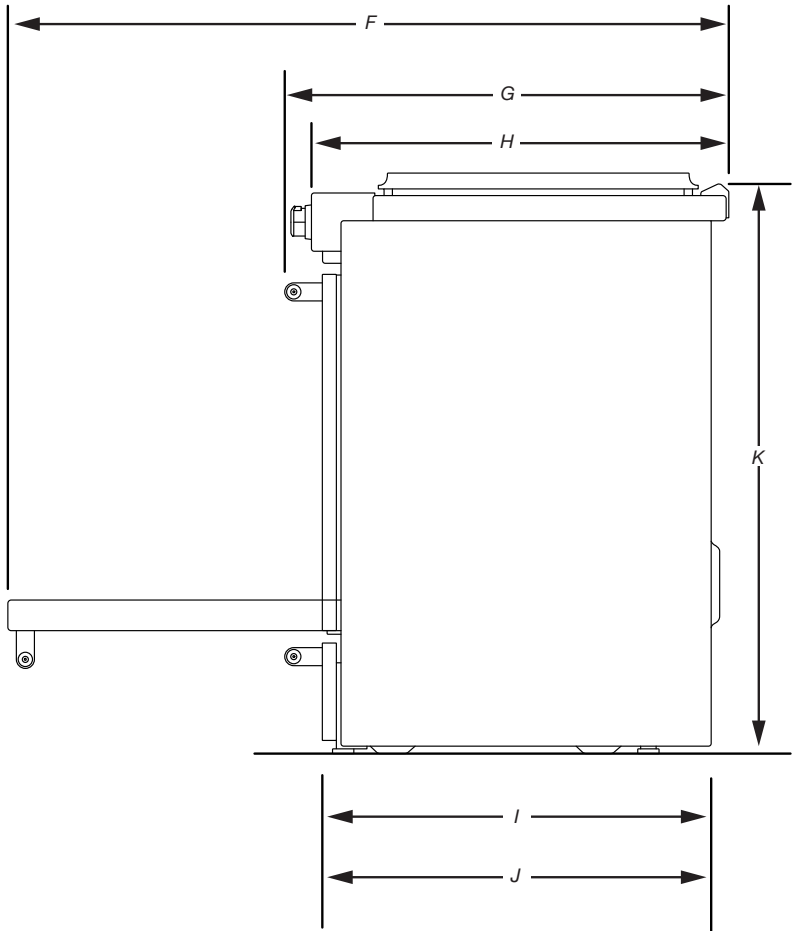
SIDE VIEW
