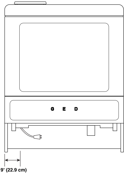
BACK VIEW
