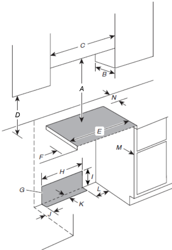
Slide-In Cutout
