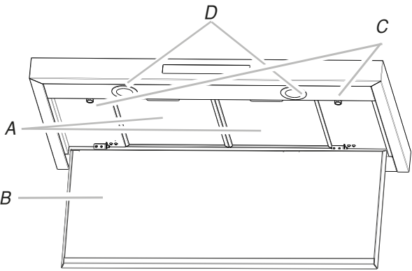
A. Metal filters B. Stainless steel panel C. Magnets (2) D. Spring catches (2)
